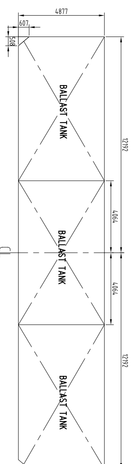
SECTION PLAN
